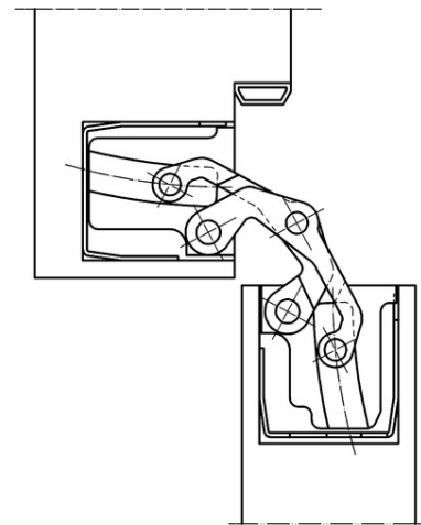
block frame 90°
