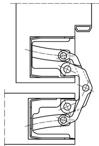
block frame 180°
